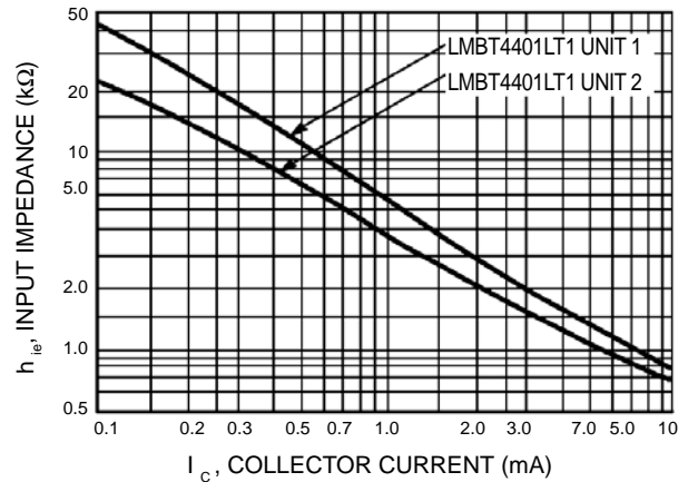
Figure 12. Input Impedance
