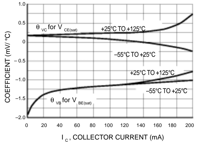
Figure 16. Temperature Coefficients
