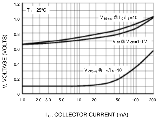
Figure 17. "ON" Voltages
