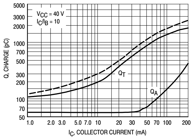
Figure 4. Charge Data
